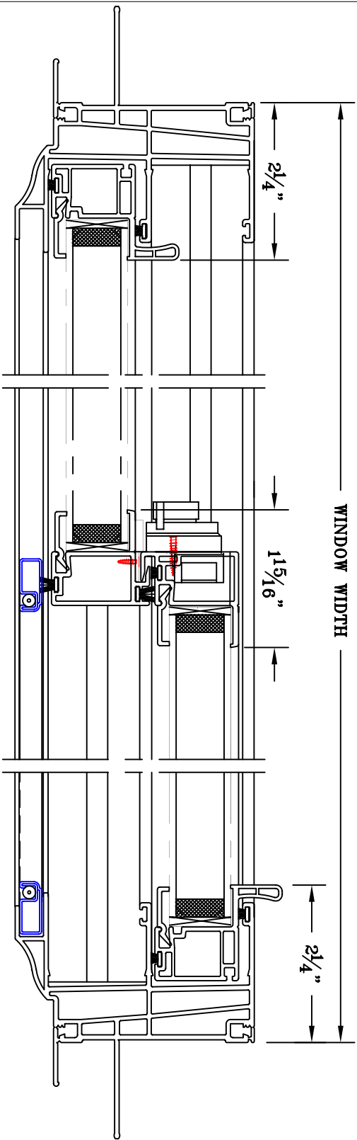
FULLY WELDED VINYL WINDOW NEW CONSTRUCTION SLIDER #CVS-420 TOP VIEW (1:2)
