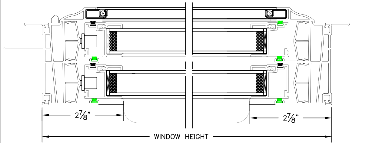
FULLY WELDED VINYL WINDOW NEW CONSTRUCTION SLIDER #CVS-420 SIDE VIEW (1:2)
