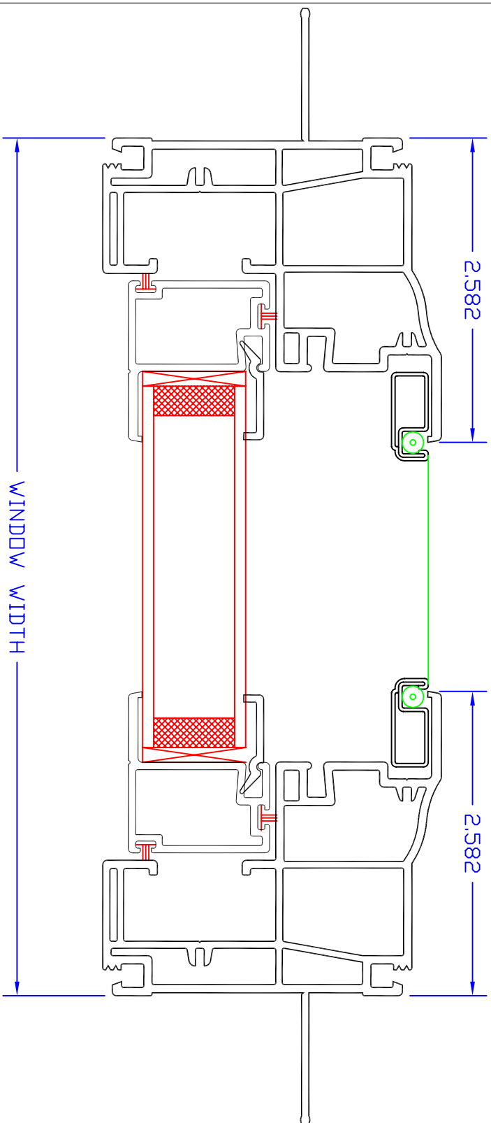
FULLY WELDED VINYL WINDOW NEW CONSTRUCTION HOPPER DOWN #CVS-340 TOP VIEW (1:1)
