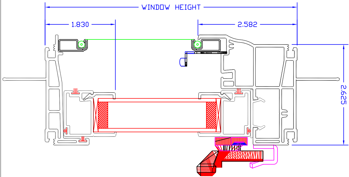
FULLY WELDED VINYL WINDOW NEW CONSTRUCTION HOPPER DOWN #CVS-340 SIDE VIEW (1:1)
