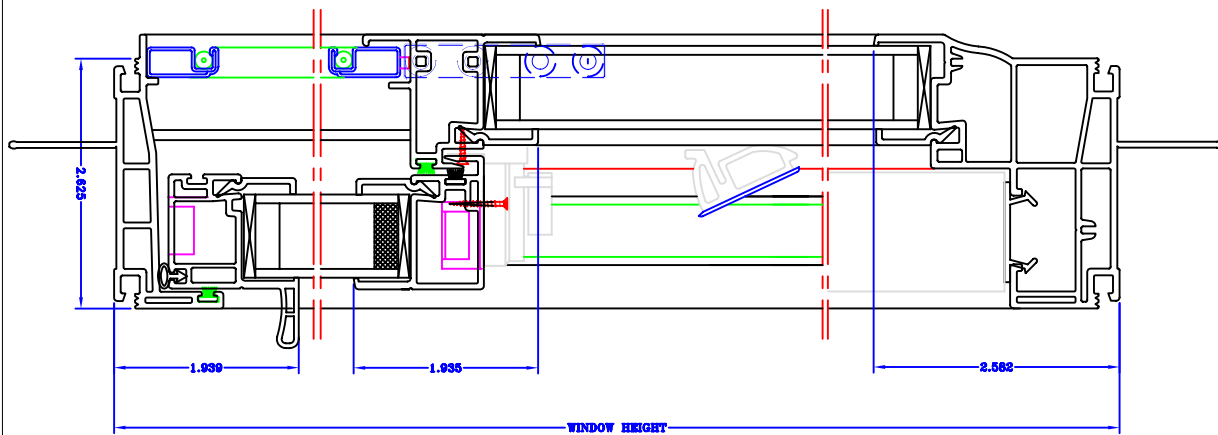
FULLY WELDED VINYL WINDOW NEW CONSTRUCTION SINGLE HUNG TILT #CVS-300 SIDE VIEW (1:1)
