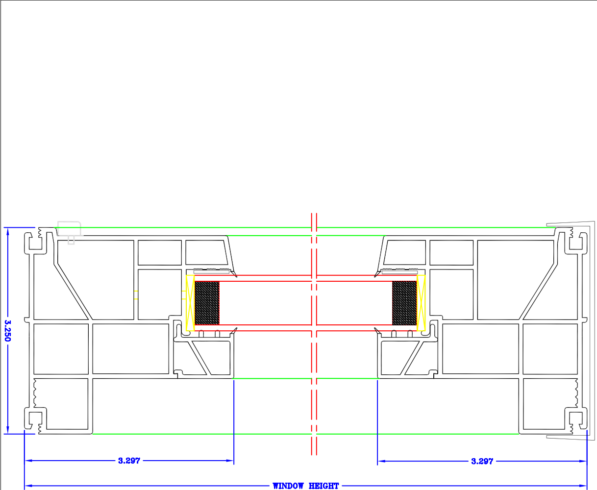
FULLY WELDED VINYL WINDOW PICTURE #CVP-210 SIDE VIEW (1:1)
