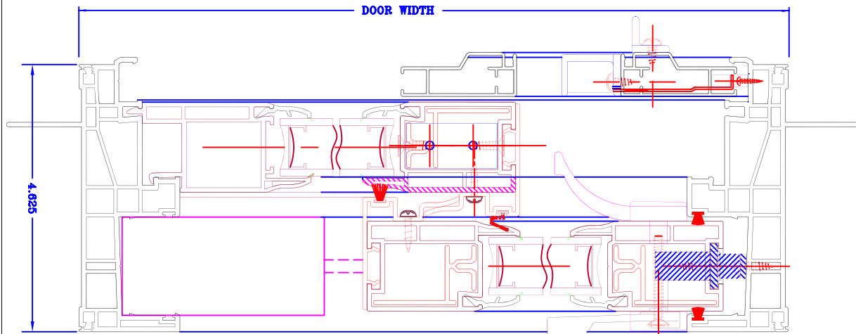
WELD VINYL PATIO SLIDING DOOR #CVP-1500 TOP VIEW (1:1)
