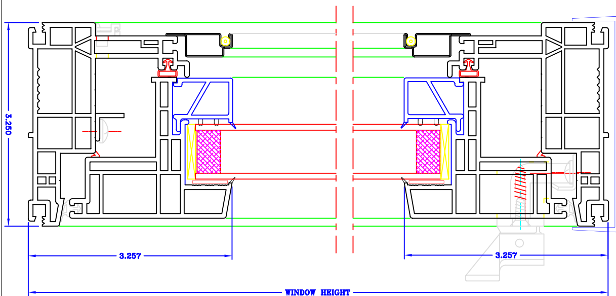
FULLY WELDED VINYL WINDOW HOPPER #CVH-250 SIDE VIEW (1:1)
