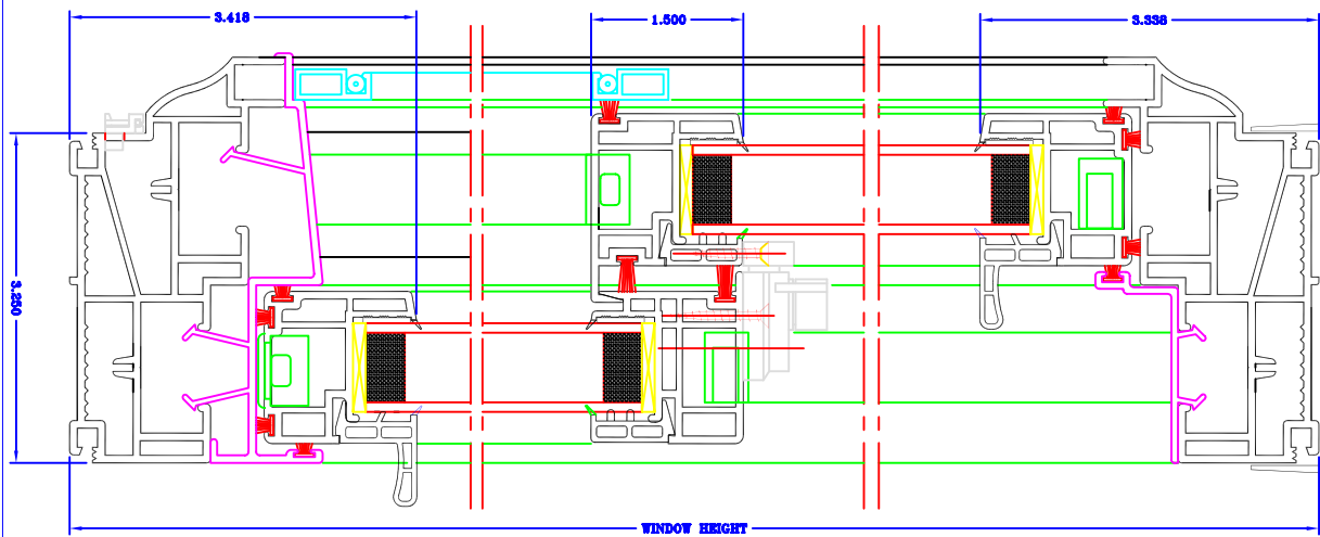
FULLY WELDED VINYL WINDOW DOUBLE HUNG TILT #CVD-200 SIDE VIEW (1:1)
