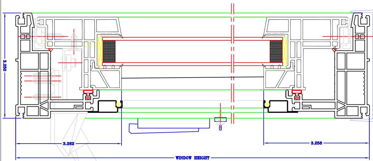
FULLY WELDED VINYL WINDOW CASEMENT #CVC-230 SIDE VIEW (1:1)
