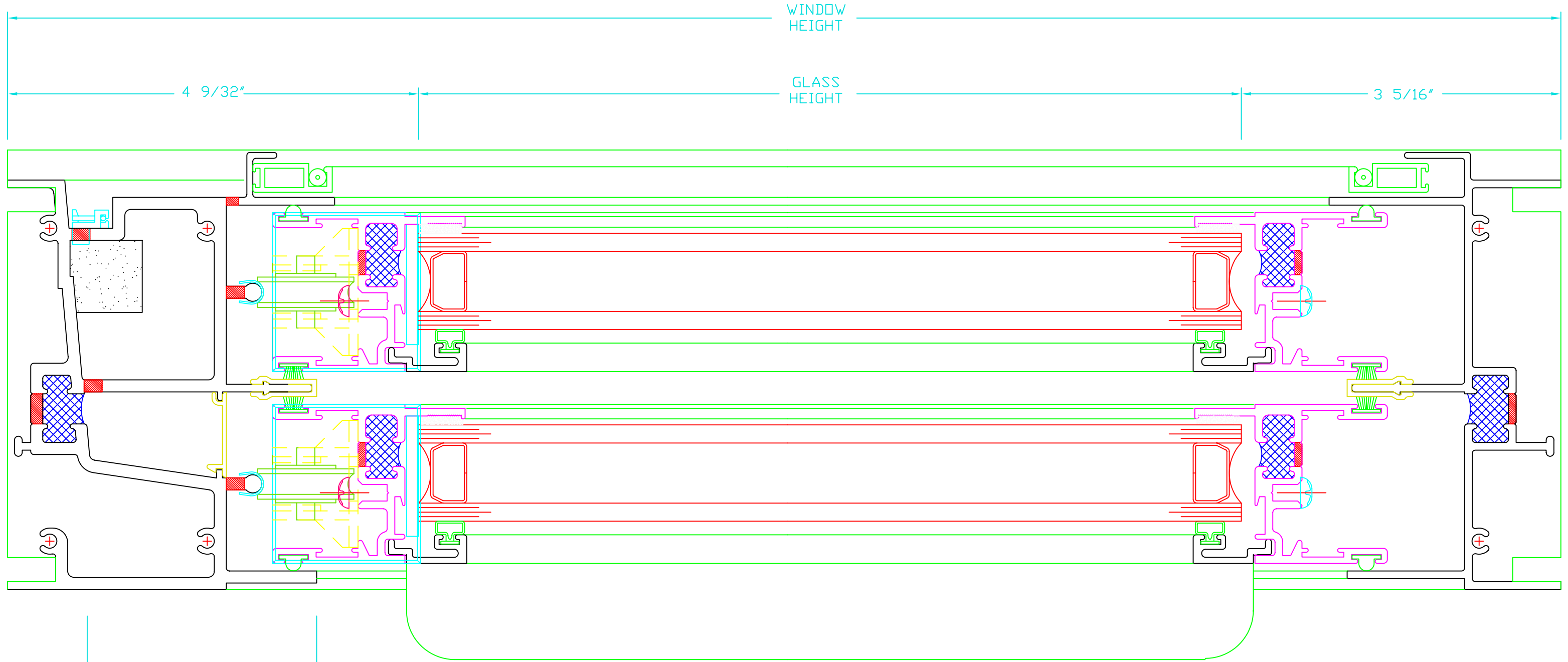
THERMAL BREAK ALUMINUM WINDOW HORIZONTAL SLIDER #CTS-6200 SIDE VIEW (I:I)
