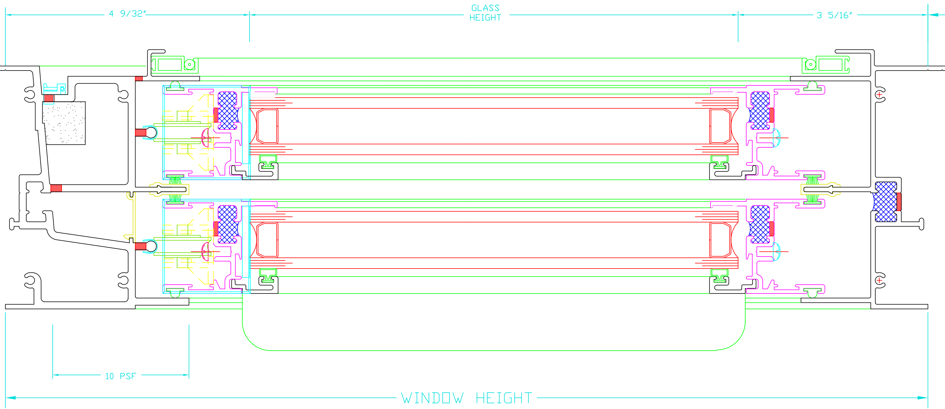
THERMAL BREAK ALUMINUM WINDOW HORIZONTAL SLIDER #CTS-6200 W/2.5 CASEMENT FIN SIDE VIEW (1:1)
