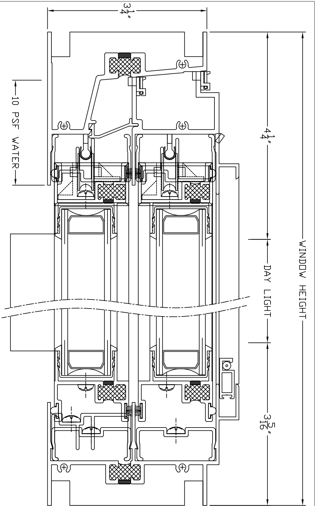
THERMAL BREAK ALUMINUM WINDOW HORIZONTAL SLIDER #CTS-5600 SIDE VIEW (1:1)
