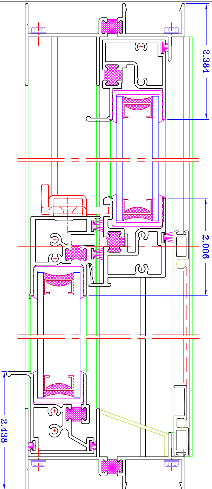
THERMAL BREAK ALUMINUM WINDOW SLIDER #CTS-2300 TOP VIEW (1:1)
