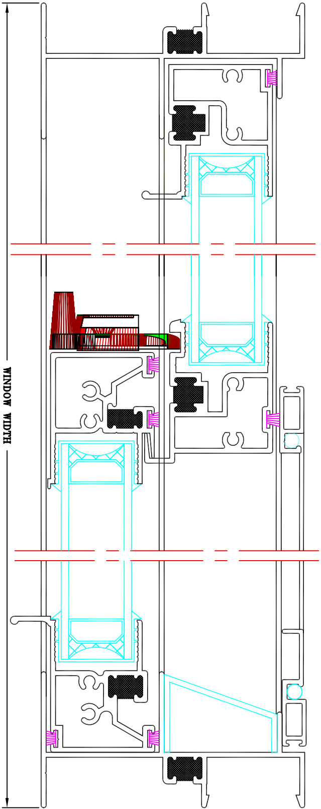
THERMAL BREAK ALUMINUM WINDOW SLIDER #CTS-2200 TOP VIEW (1:1)
