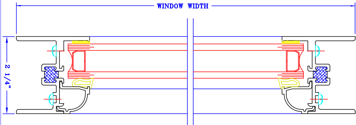
ALUMINUM PICTURE Series #CTC-8100 TOP VIEW (1:1)
