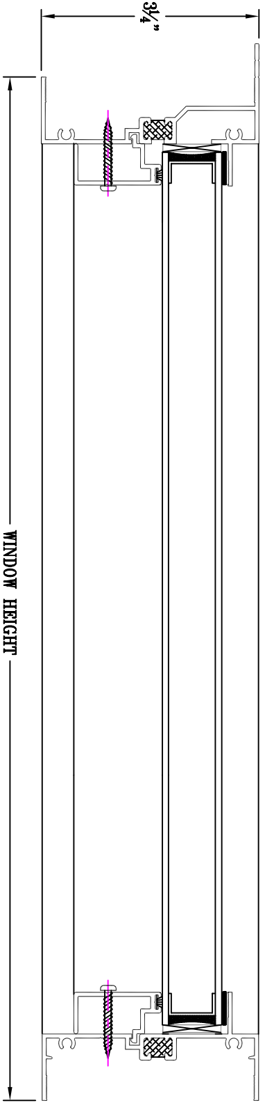
THERMAL BREAK ALUMINUM WINDOW PICTURE #CTP-2100 SIDE VIEW (1:2)
