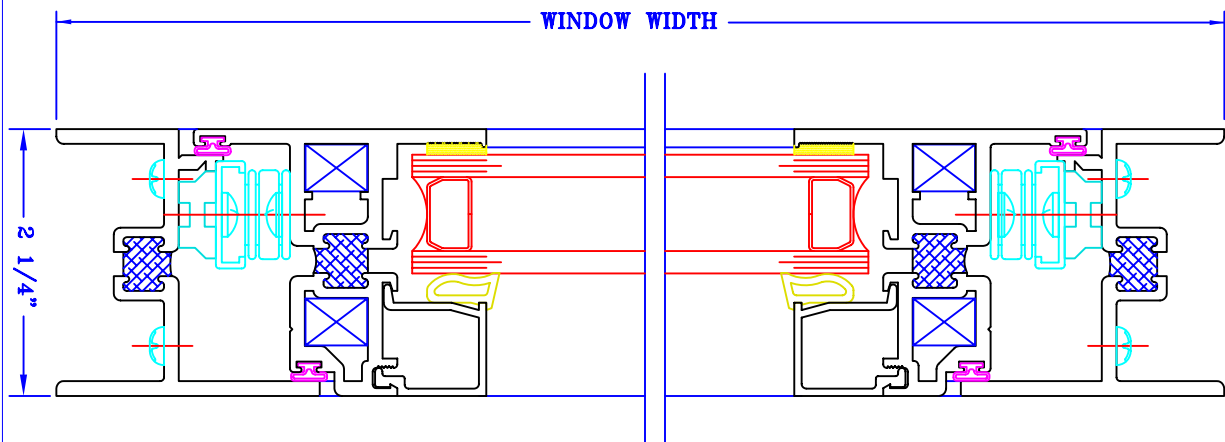
ALUMINUM PROJECT OUT Series #CTC-8200 TOP VIEW (1:1)
