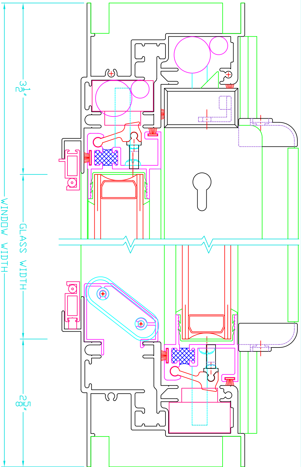
THERMAL BREAK ALUMINUM WINDOW DOUBLE HUNG TILT #CTD-5500 TOP VIEW (1:1)
