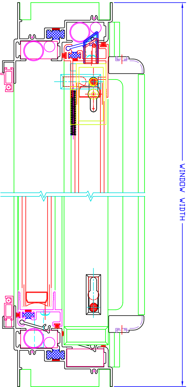
THERMAL BREAK ALUMINUM WINDOW DOUBLE HUNG TILT #CTD-5000 TOP VIEW (1:2)
