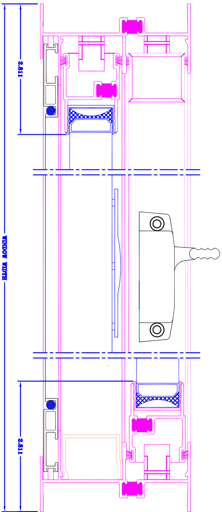
THERMAL BREAK ALUMINUM WINDOW SIDE LOAD DOUBLE HUNG #CTD-3000 TOP VIEW (1:1)
