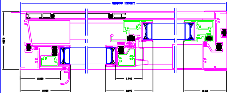
THERMAL BREAK ALUMINUM WINDOW SIDE LOAD DOUBLE HUNG #STD-30100 SIDE VIEW (1:1)
